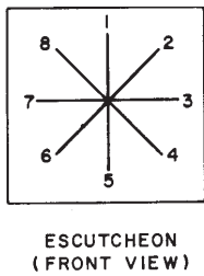
Figure 12B: Contact arrangements to meet cam limitations
