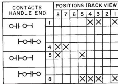
Figure 12B: Contact arrangements to meet cam limitations
