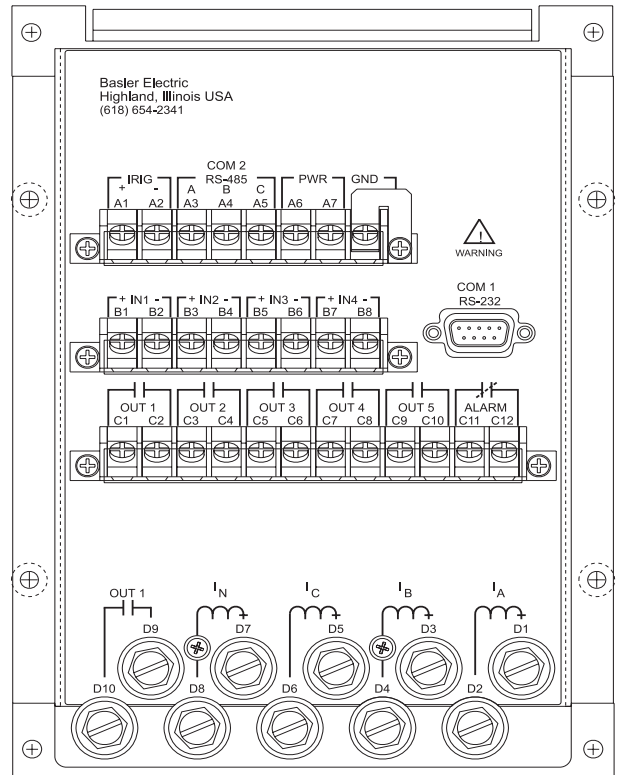
Figure 5C - BE1-851 S1 Rear Panel Connections
