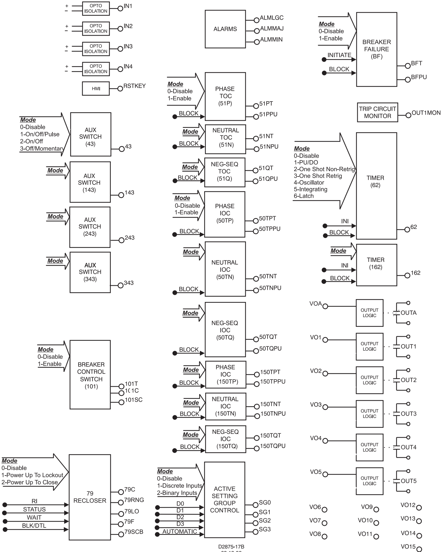
Figure 6B - BESTlogic Sensing Input Type H Function Blocks
